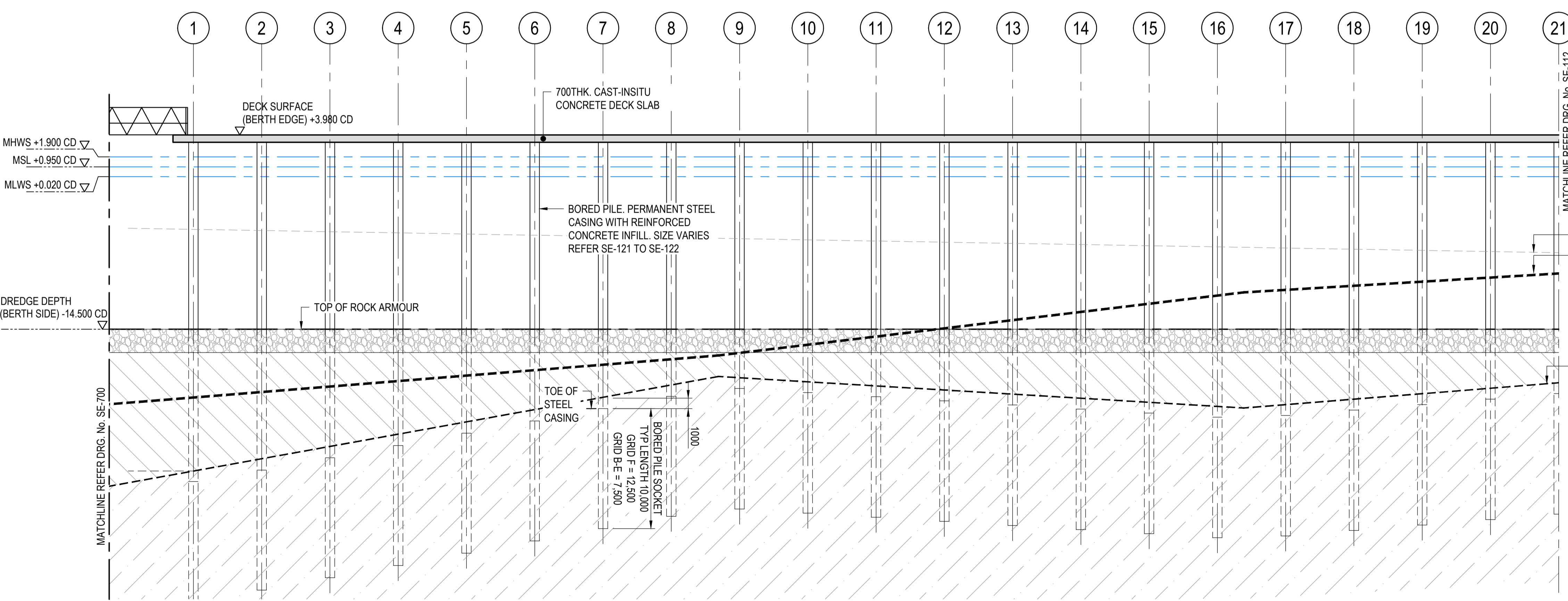
GENERAL ARRANGEMENT - PARTIAL ELEVATION 1:250
