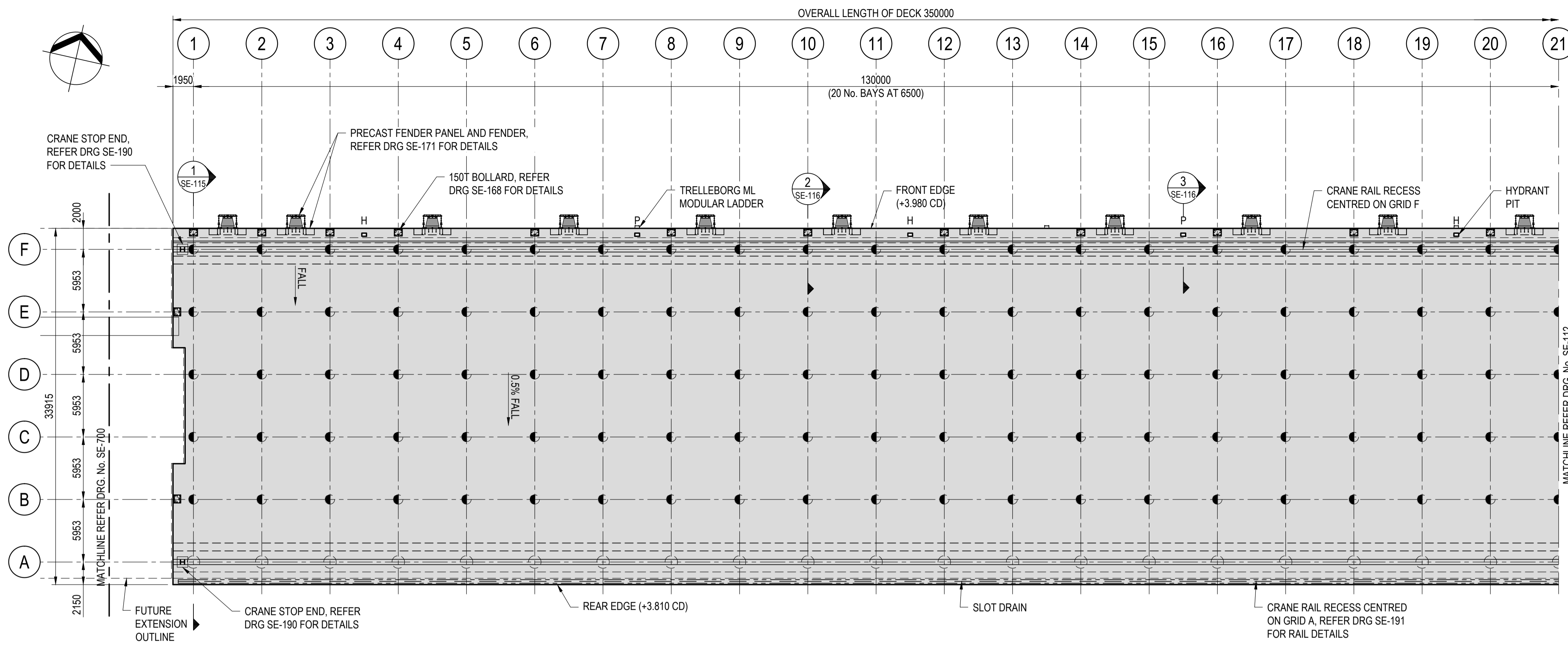
GENERAL ARRANGEMENT - PARTIAL PLAN 1:250
