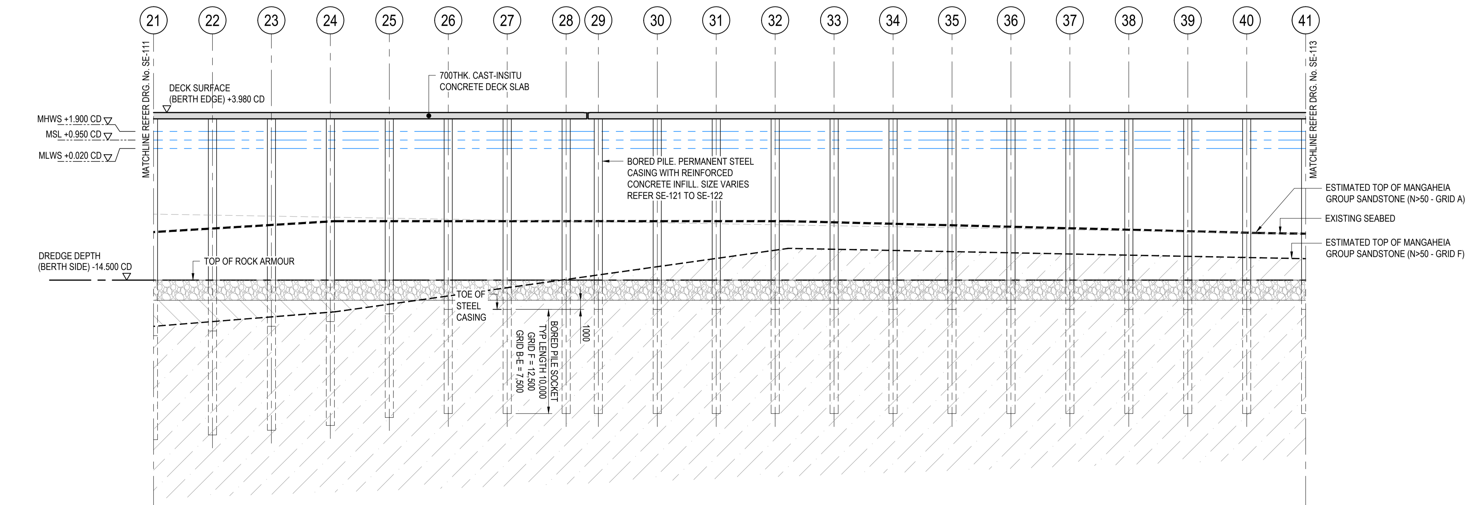
GENERAL ARRANGEMENT - PARTIAL ELEVATION 1:250
