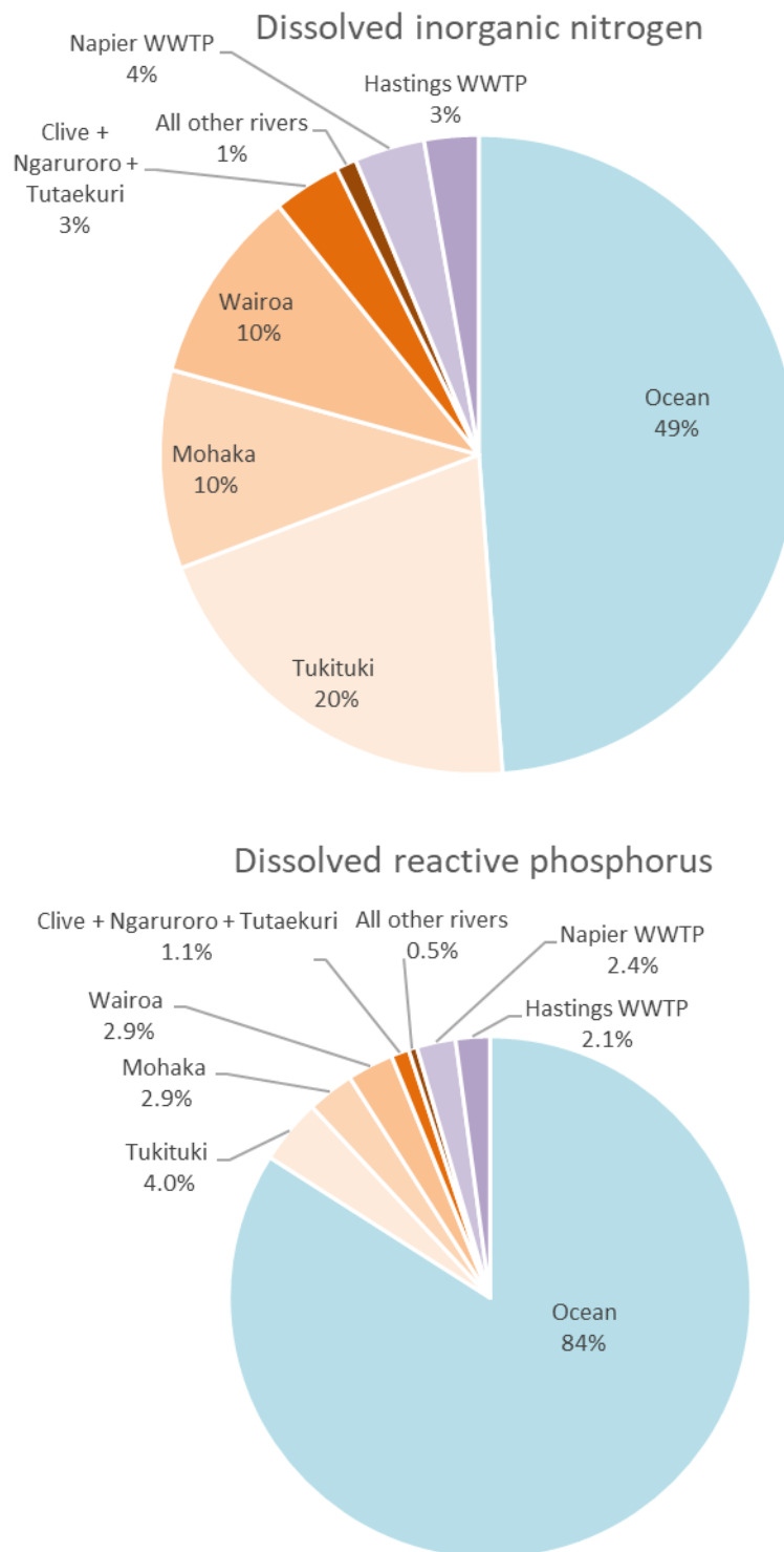
Figure 3-9: Relative contributions of potential dissolved inorganic nitrogen and potential dissolved reactive phosphorus in Hawke Bay from different sources.
