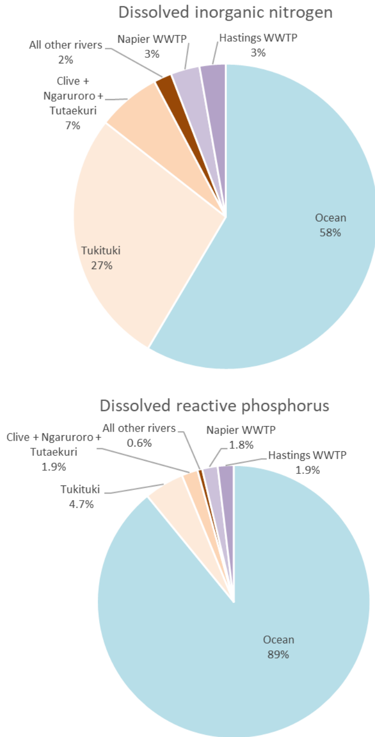
Figure 3-13: Relative contributions of potential dissolved inorganic nitrogen and potential dissolved reactive phosphorus off Cape Kidnappers from different sources.
