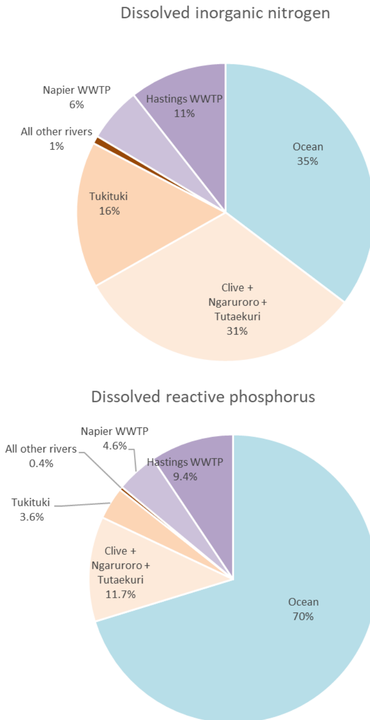
Figure 3-12: Relative contributions of potential dissolved inorganic nitrogen and potential dissolved reactive phosphorus off Awatoto from different sources.
