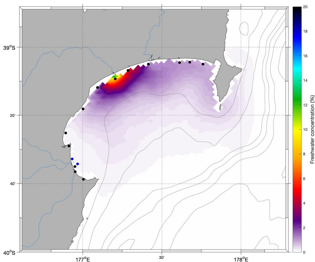
Figure 3-2: Time-averaged surface concentration for tracers released at the Mohaka River for the simulation period January 2017-December 2017. The surface concentration is expressed as a percentage of the total freshwater entering Hawke Bay.
