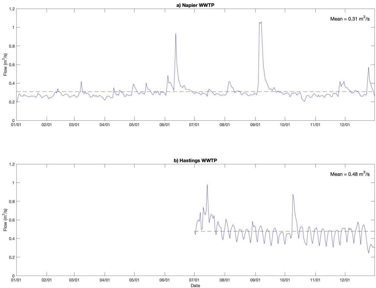
Figure 2-3: Freshwater flow rate time series for the two wastewater outfalls in Hawke Bay. The dashed horizontal line represents the annual mean flow.
