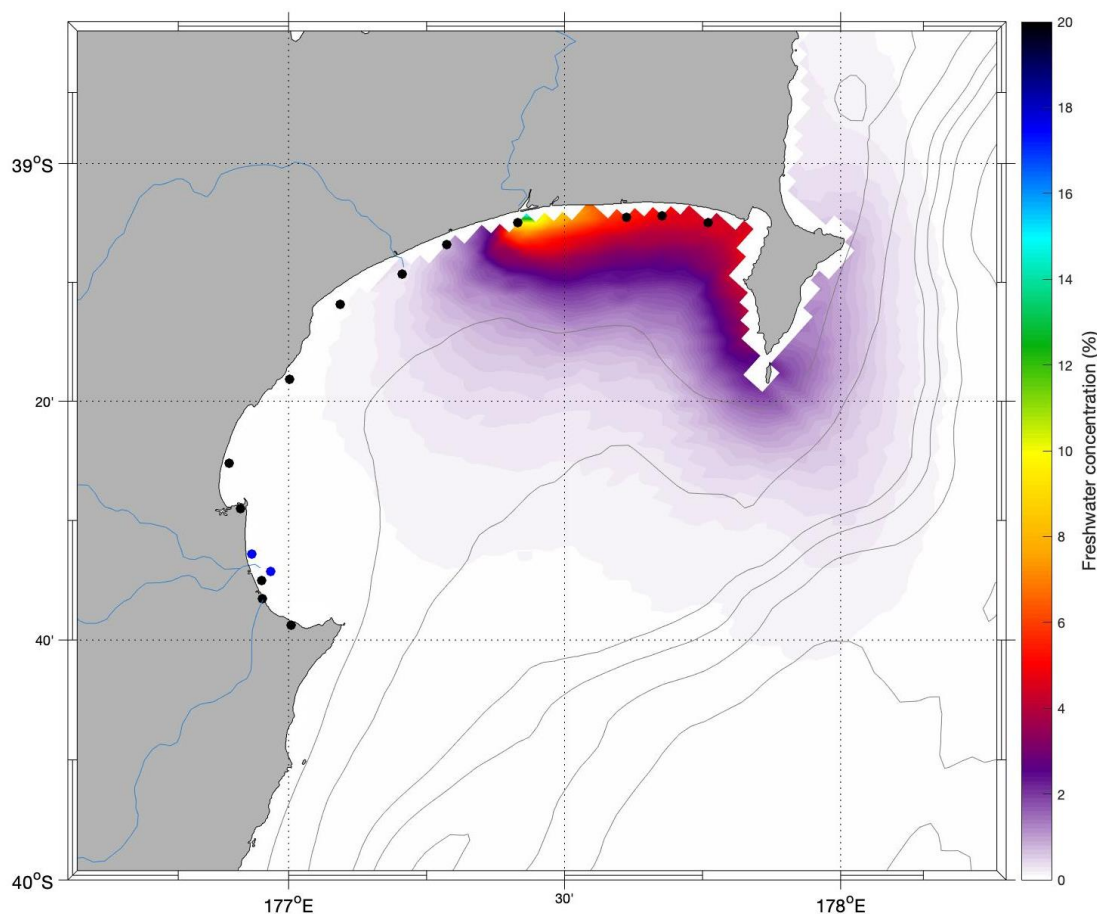
Figure 3-3: Time-averaged surface concentration for tracers released at the Wairoa River for the simulation period January 2017-December 2017. The surface concentration is expressed as a percentage of the total freshwater entering Hawke Bay.
