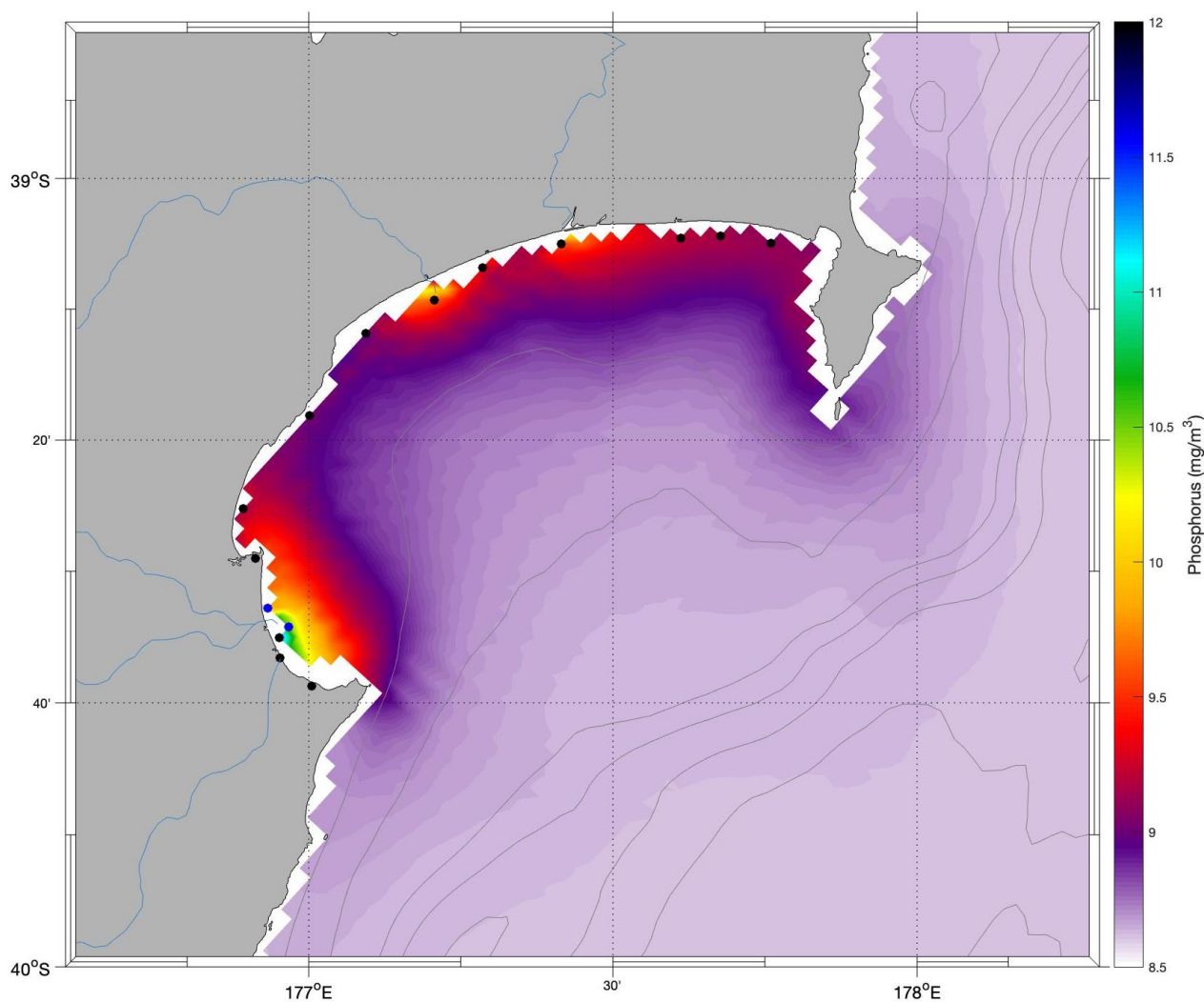
Figure 3-8: Time averaged surface concentrations of dissolved reactive phosphorus in Hawke Bay. The phosphorus concentration was calculated as the sum of the background oceanic DRP and the DRP concentrations originating from each source. The latter was estimated by multiplying the water volume fraction in the bay originating from each source by the mean DRP concentration in that source. A background oceanic DRP concentration of 8.6 mg/m 3 is assumed, based on the CARS2009 climatology.
