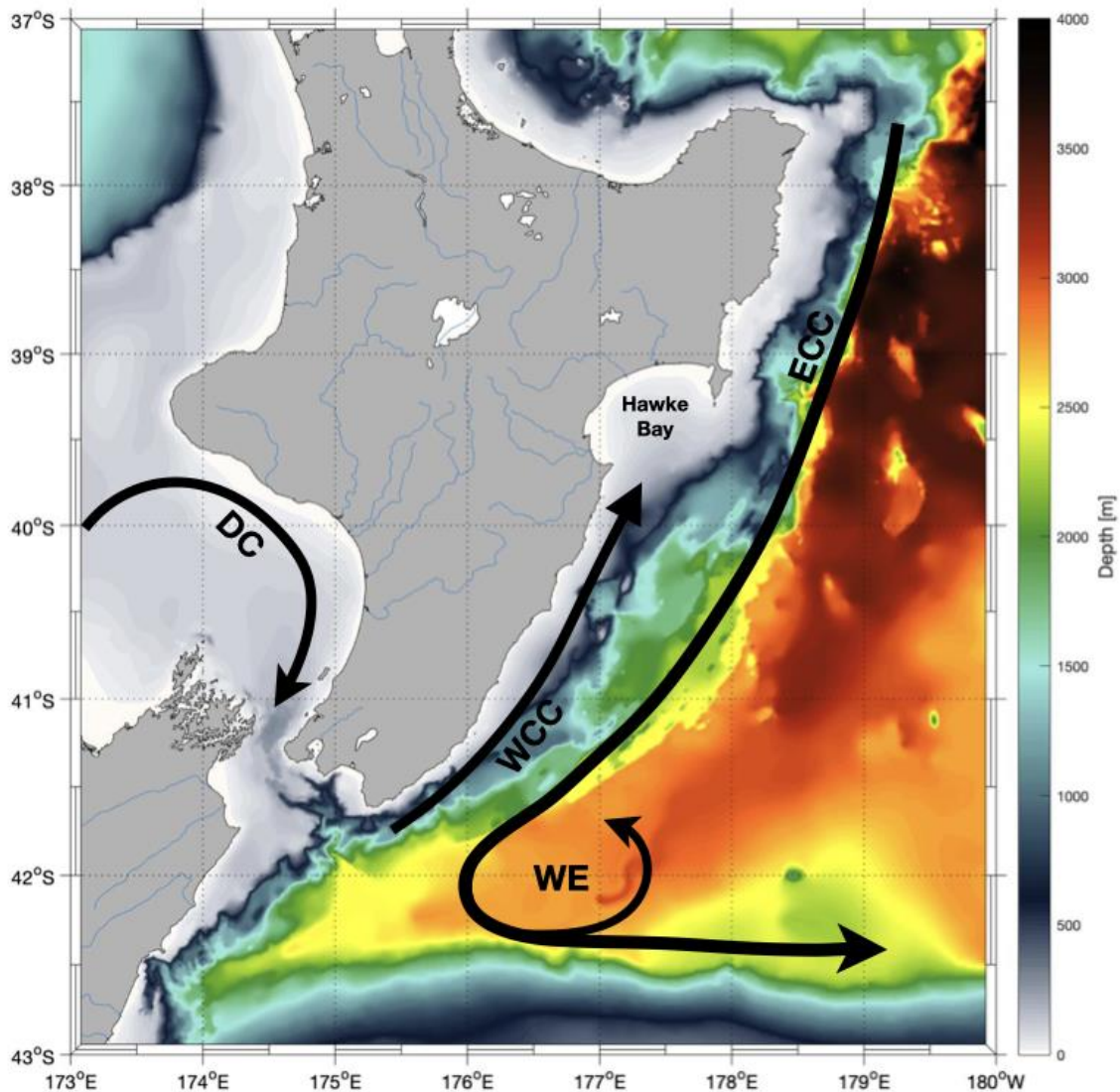
Figure 1-1: Schematic of the circulation along the east coast of the North Island. The following circulation features are indicated by the black arrows: the East Cape Current (ECC), the Wairarapa Coastal Current (WCC), the Wairarapa Eddy (WE), and the D'Urville Current (DC) in Cook Strait.
