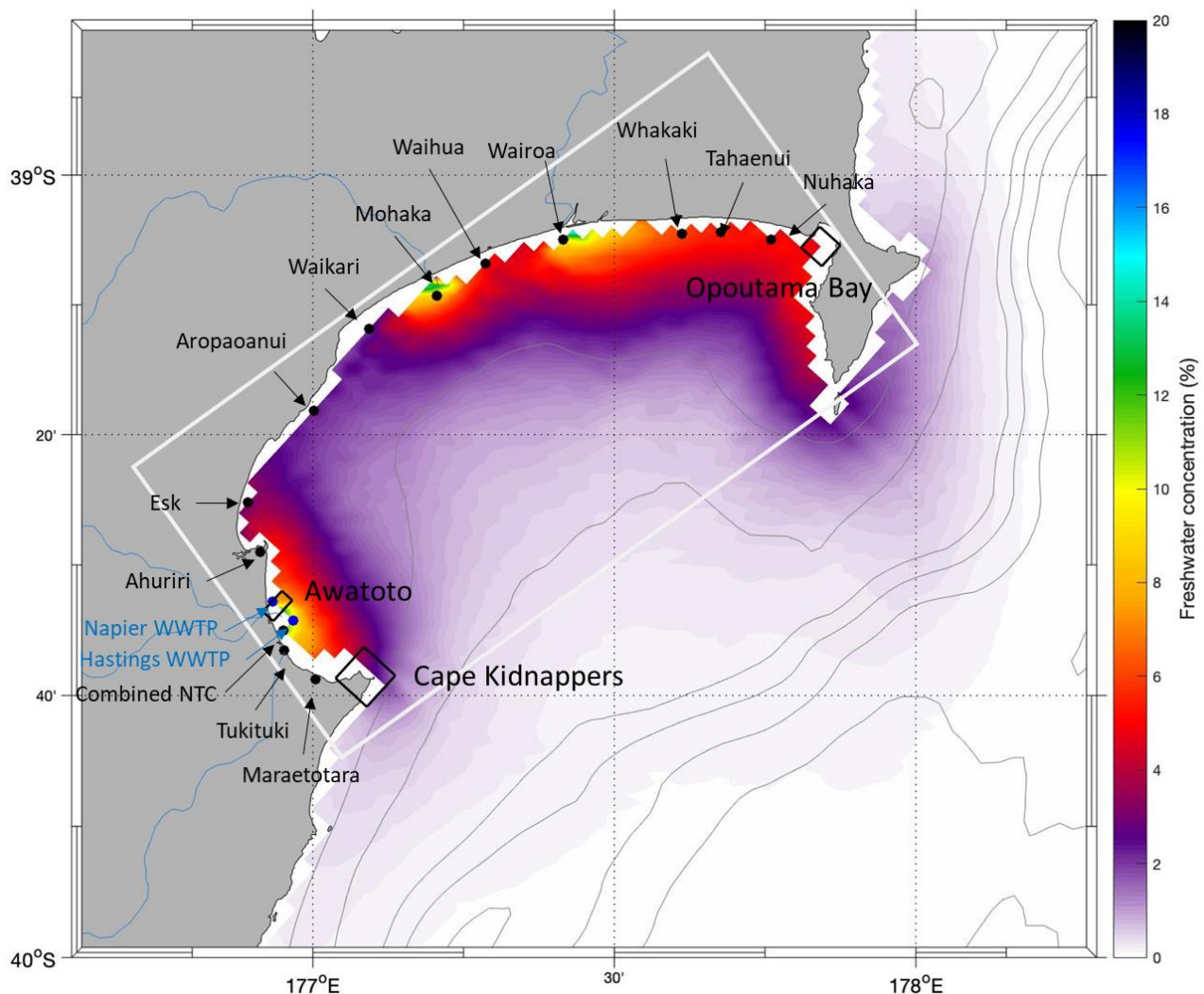
Figure 3-1: Time-averaged surface freshwater concentration for the simulation period January 2017-December 2017. The white box delineates the area considered as Hawke Bay. The black boxes indicate specific areas of interest in Hawke Bay: (from north to south) Opoutama Bay, Awatoto, Cape Kidnappers.
