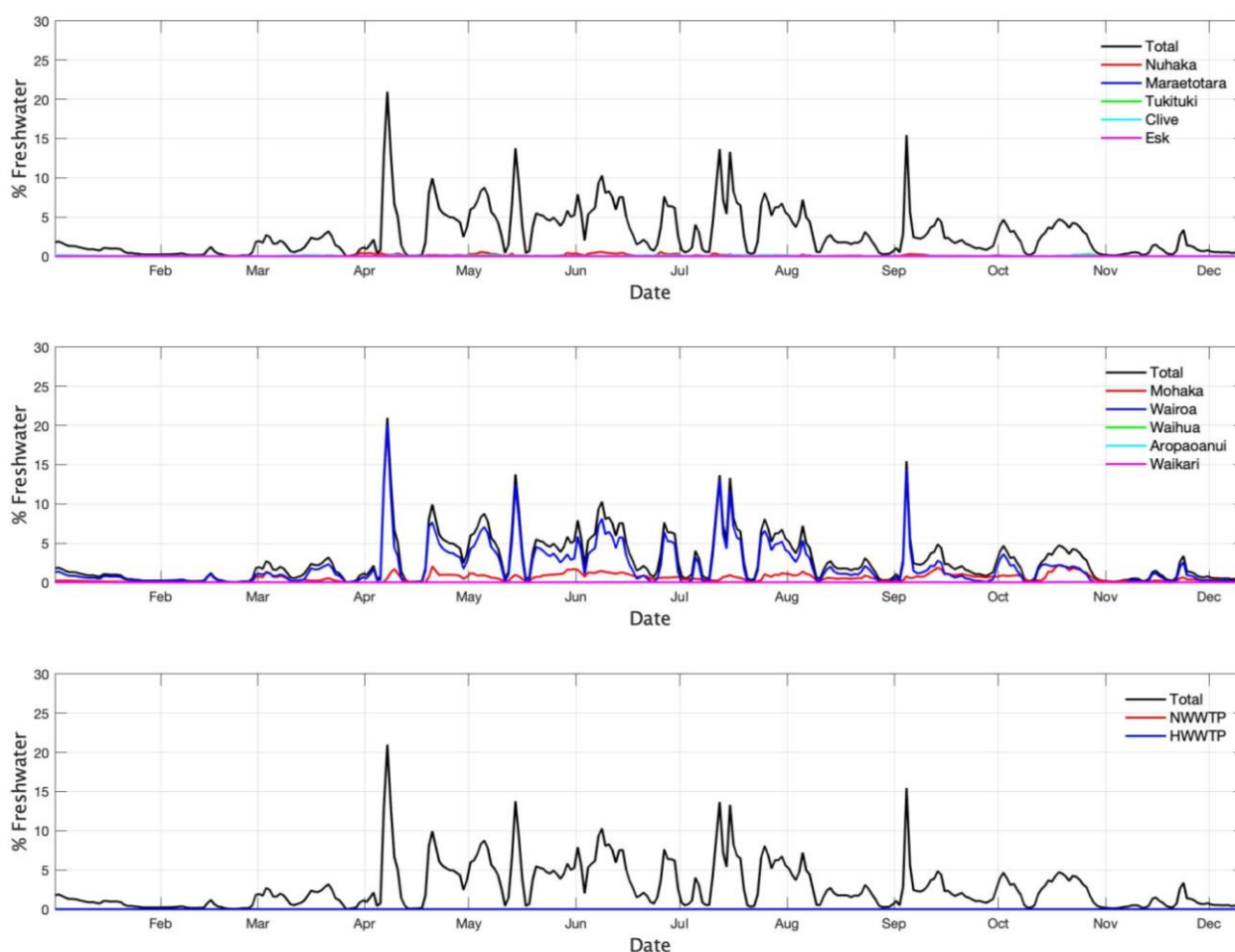
Figure 3-6: The percentage of freshwater from different rivers (top and middle) and two wastewater outfalls (bottom) contributing to the freshwater in Oputama Bay. The time-series are the volume-averaged tracer concentration averaged over the black box for Oputama Bay in Figure 3-1. Clive includes the Ngaruroro and Tutaekuri Rivers.
