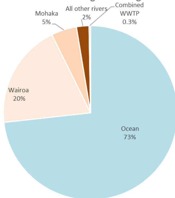
Figure 3-11: Relative contributions of potential dissolved inorganic nitrogen and potential dissolved reactive phosphorus in Opoutoma Bay from different sources.
