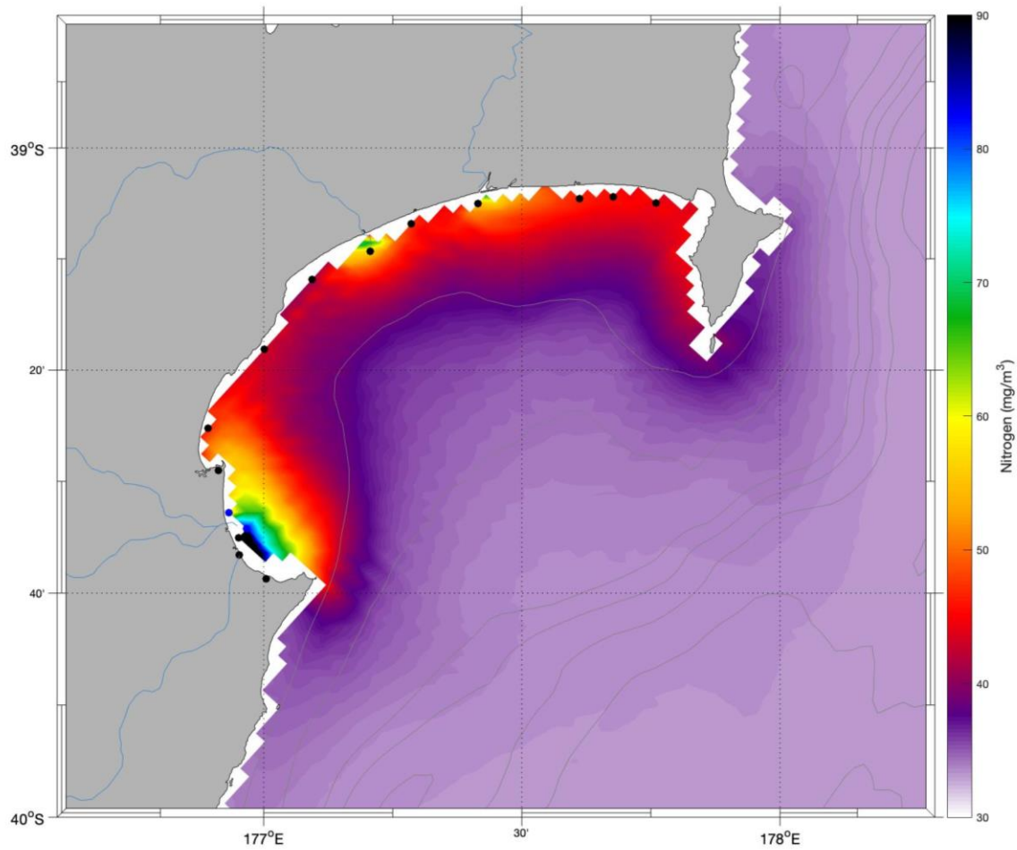
Figure 3-7: Time-averaged surface concentrations of dissolved inorganic nitrogen in Hawke Bay. The nitrogen concentration was calculated as the sum of the background oceanic DIN and the DIN concentrations originating from each source. The latter was estimated by multiplying the water volume fraction in the bay originating from each source by the mean DIN concentration in that source. A background oceanic DIN of 33.1 \text{ mg/m}^3 is assumed, based on the CARS2009 climatology.
