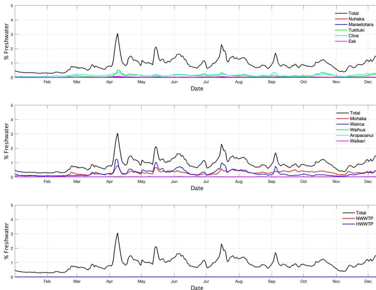
Figure 3-4: The percentage of freshwater from the different rivers (top and middle) and two wastewater outfalls (bottom) discharging into Hawke Bay . The time-series are the volume-averaged tracer concentration averaged over the white box in Figure 3-1. Clive includes the Ngaruroro and Tutaekuri Rivers. Note the Total is included on all 3 panels for comparison.
