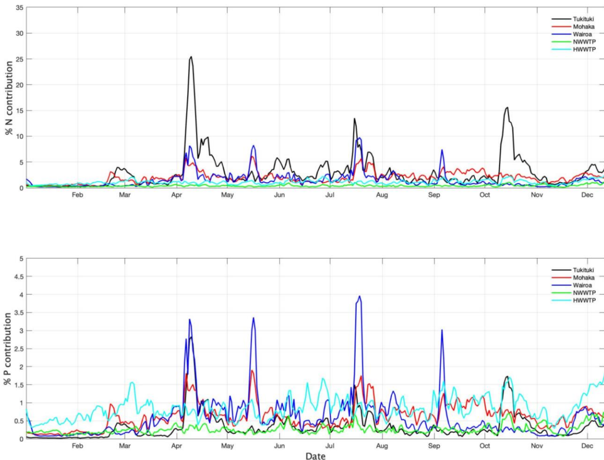
Figure 3-10: Timeseries of nitrogen (top) and phosphorus (bottom) contribution to Hawke Bay from the 5 main terrestrial sources.
