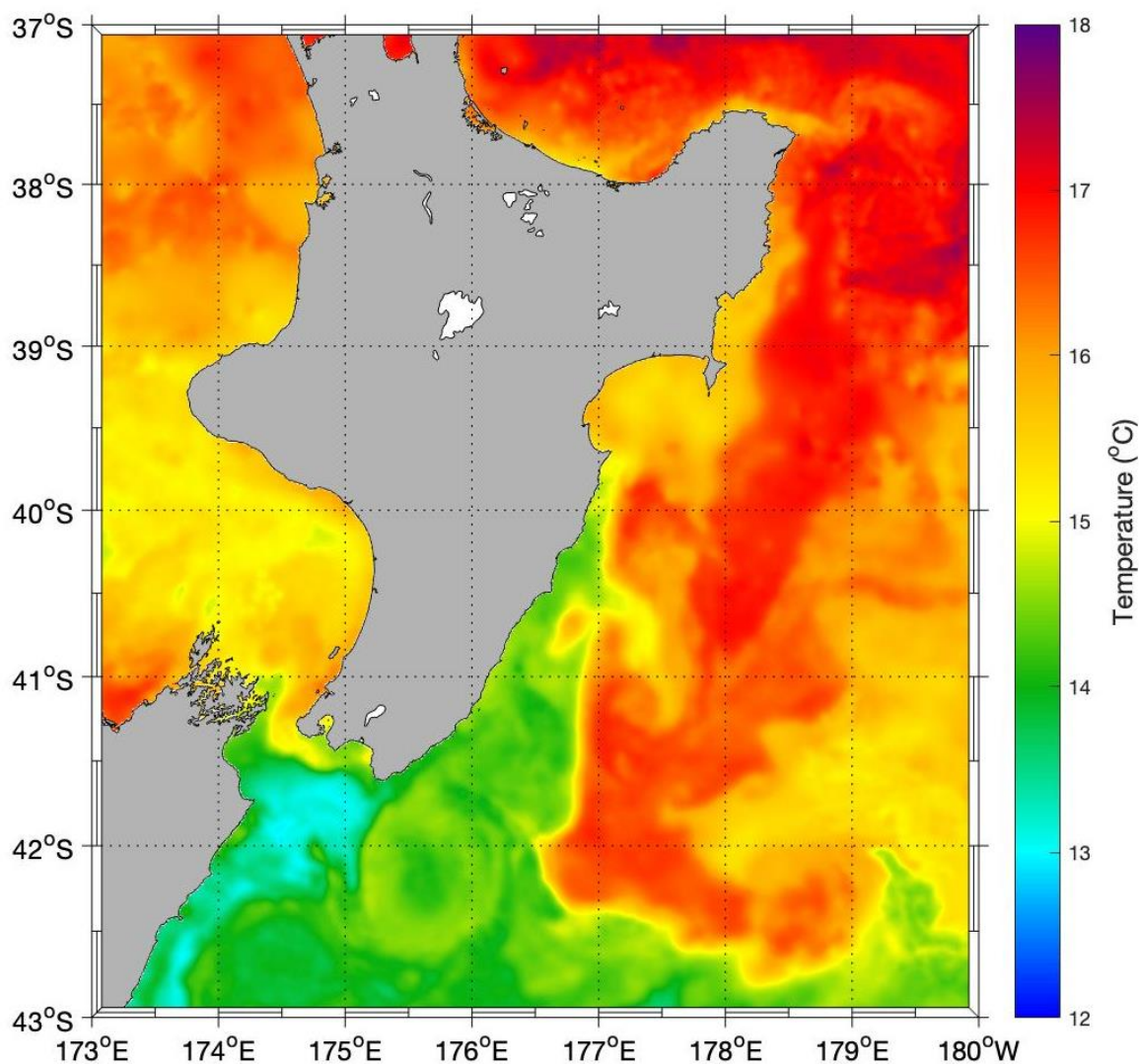
Figure 1-2: A snapshot of satellite derived sea surface temperature (SST) for 25 October 2017. The colder temperature along the east coast of the North Island is indicative of the WCC. Data source: MUR-JPL-L4-GLOB-v4.1 sourced from https://podacc.jpl.nasa.gov .
