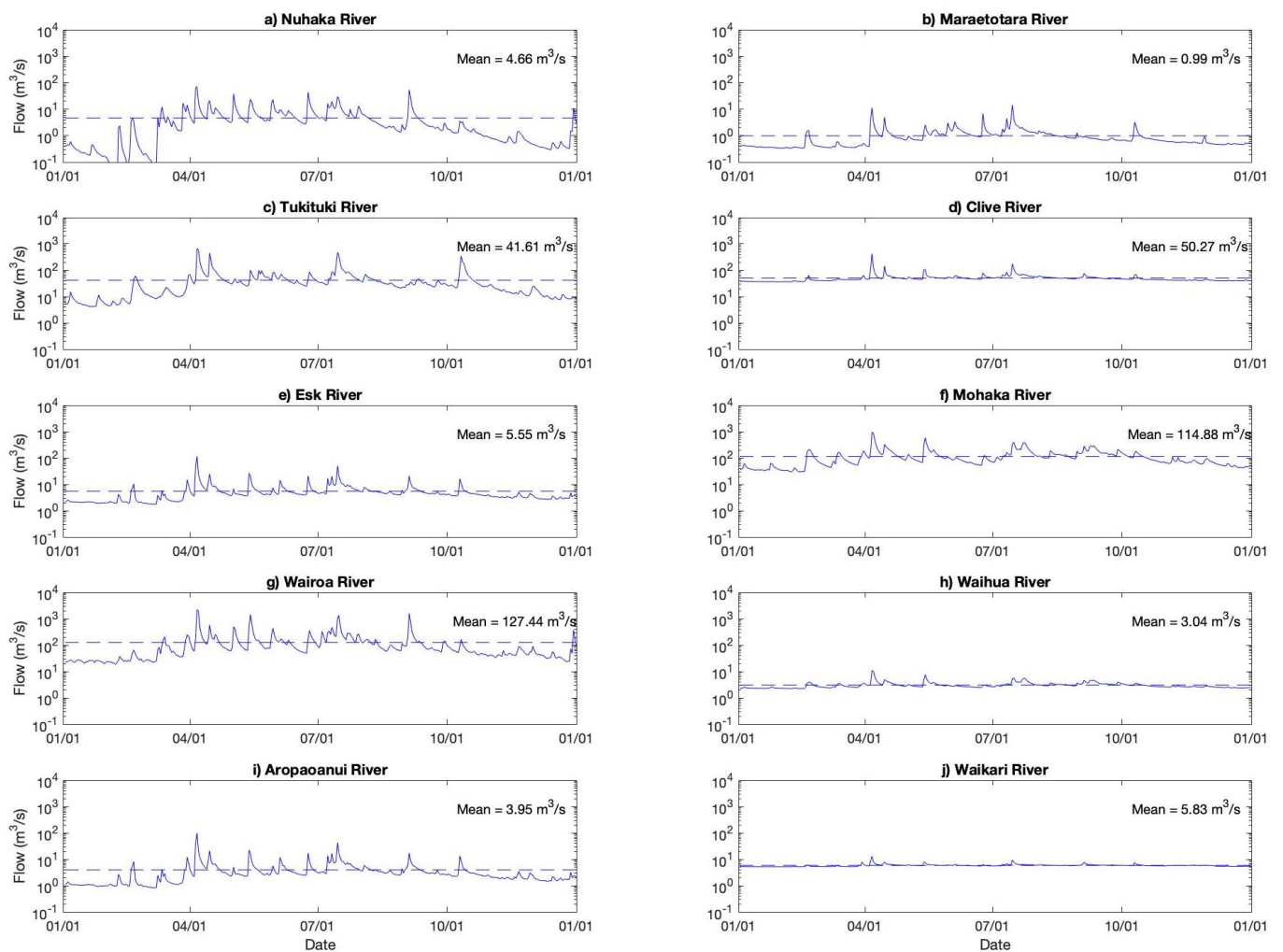
Figure 2-2: Freshwater flow rate timeseries for 10 of the rivers terminating in Hawke Bay. The flow rate is presented on a logarithmic scale. The dashed horizontal line represents the annual mean flow. The Clive River also includes the Ngaruroro and Tutaeakuri Rivers.
