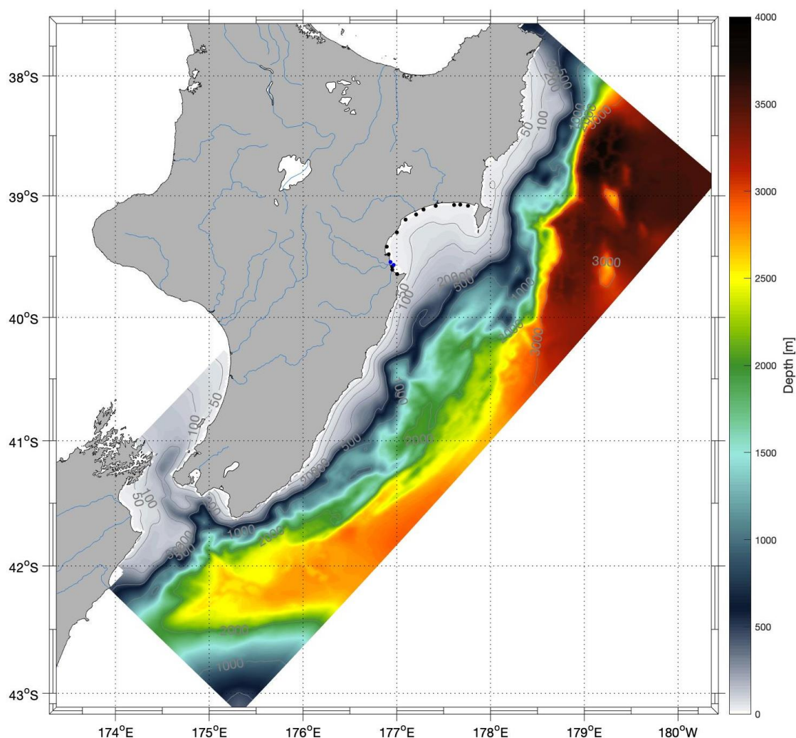
Figure 2-1: Model domain showing bathymetry in meters (m). The black dots indicate the rivers terminating along the Hawke Bay coast that were included in the model as freshwater point sources. These rivers are listed in order from North to south in Table 2-1. The blue dots indicate the two wastewater treatment plant outfalls that were also included as freshwater point sources.
