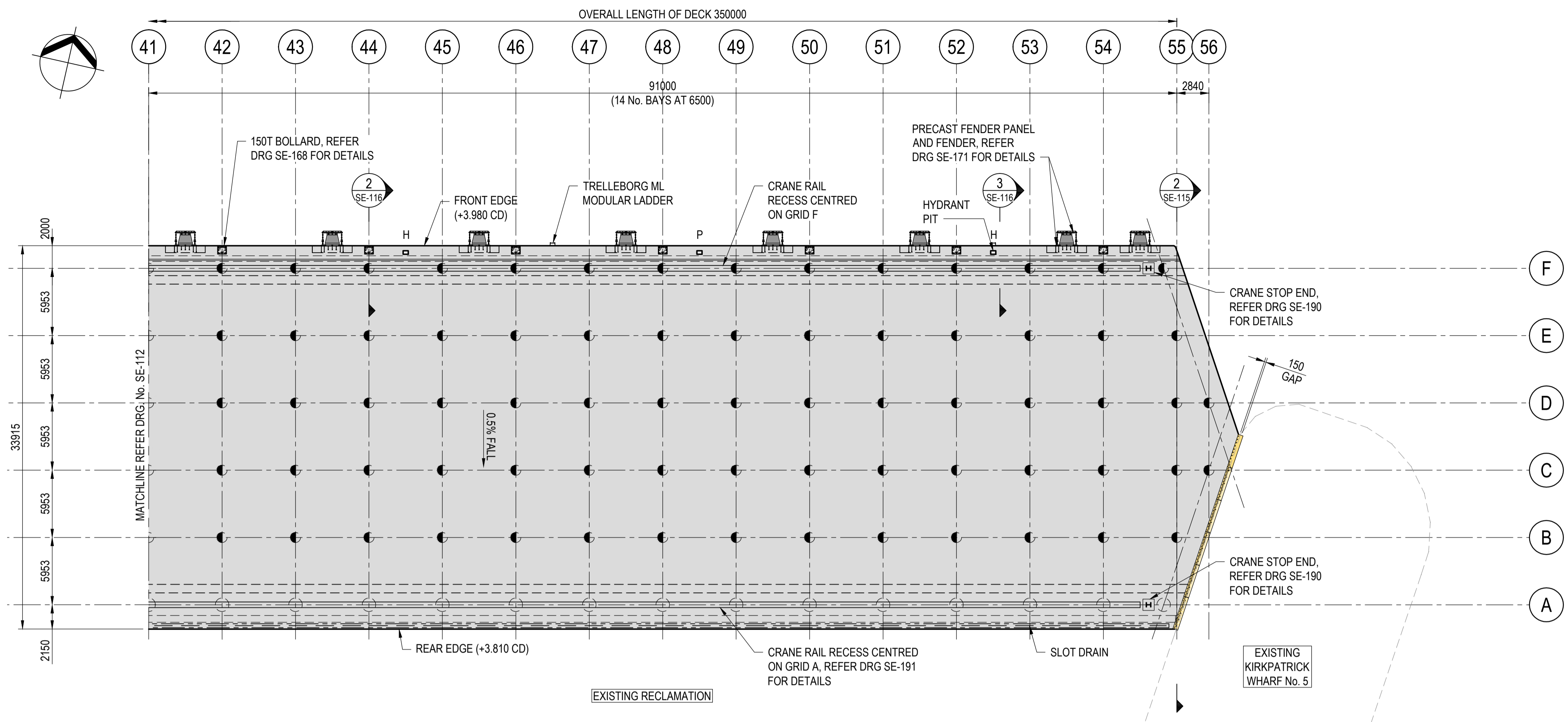
GENERAL ARRANGEMENT - PARTIAL PLAN 1:250
