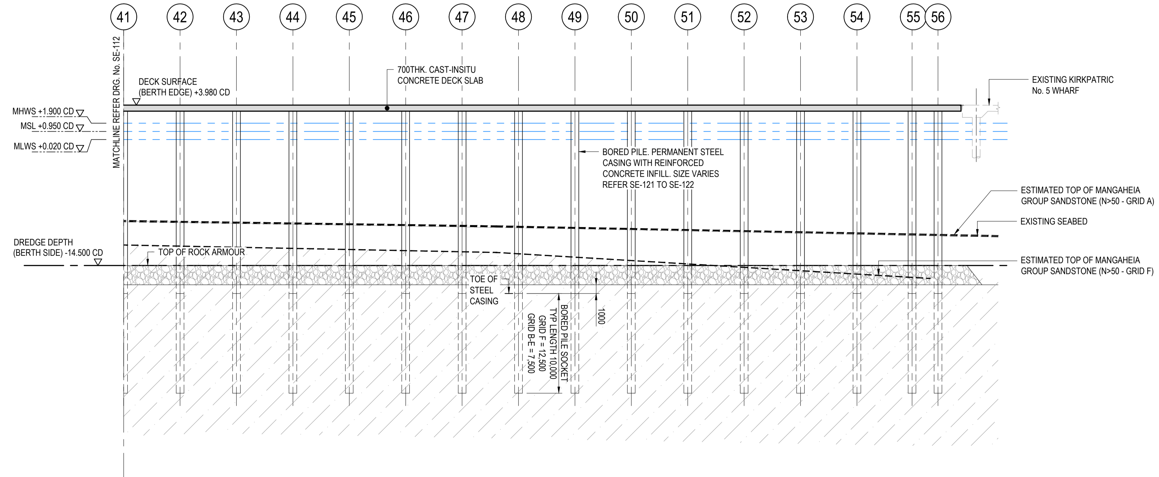
GENERAL ARRANGEMENT - PARTIAL ELEVATION 1:250
