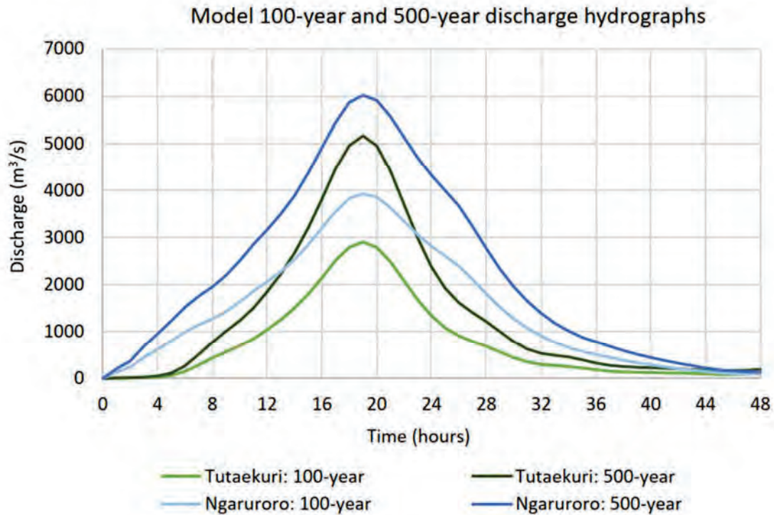
Figure 5. Example hydrograph for 100yr and 500yr ARIs in the HBRC Model.
