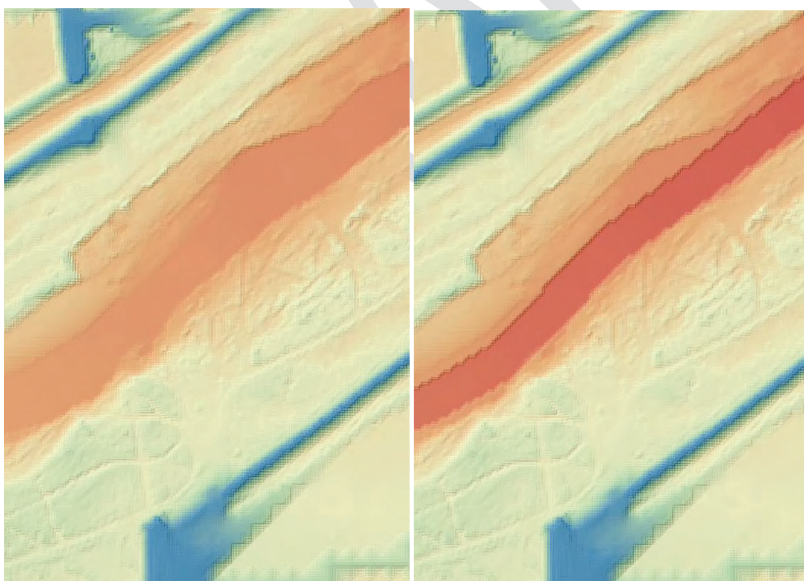
Figure 3.4: DEM modification example – river channel (left supplied DEM, right: Modified DEM).
